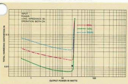
TOTAL HARMONIC DISTORTION VS OUTPUT POWER
